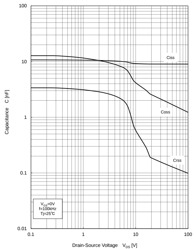
Fig.11 Capacitance (Typical)
