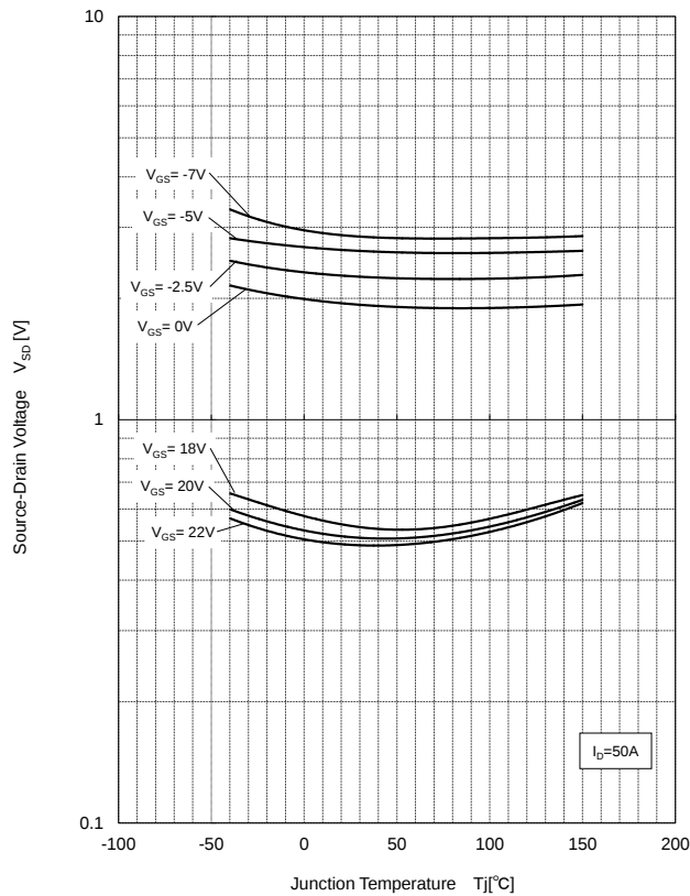
Fig.10 Source-Drain Voltage vs Junction Temperature (Typical)
