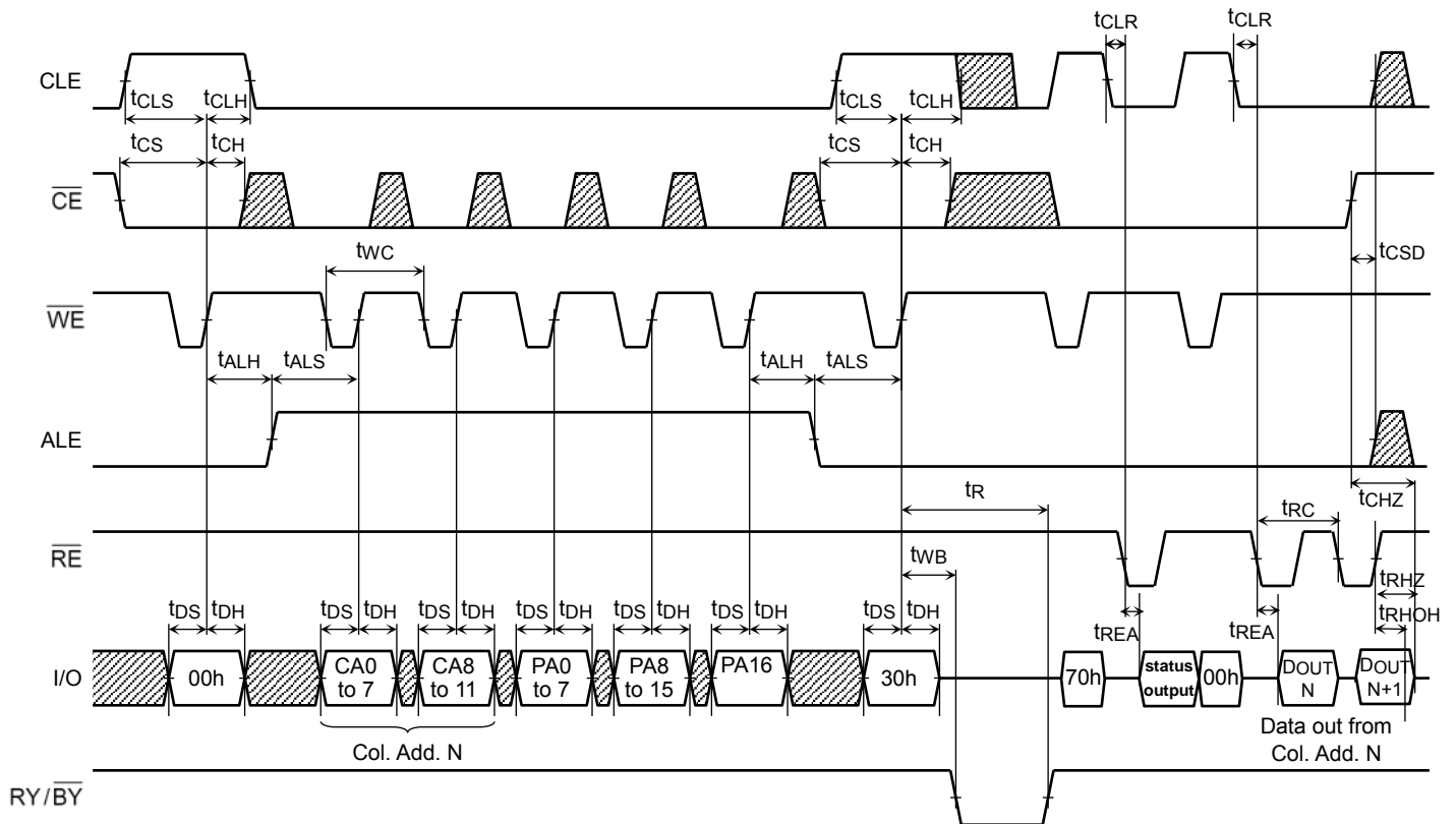
Read Cycle Timing Diagram: When Interrupted by CE
