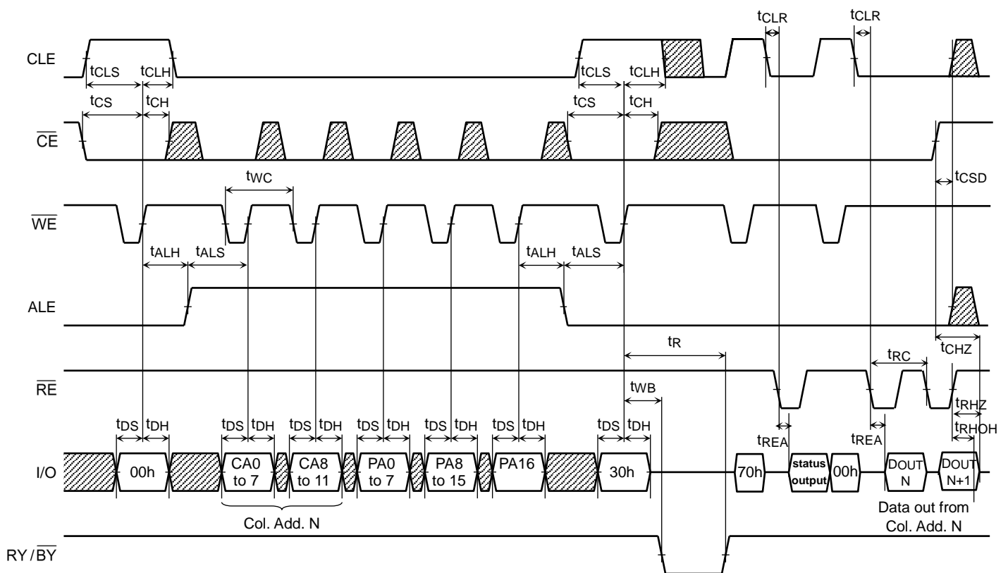
Read Cycle Timing Diagram: When Interrupted by \overline{\text{CE}}
