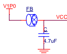
Figure 1 Noise Processing of the Input End of the V CC Core Voltage
