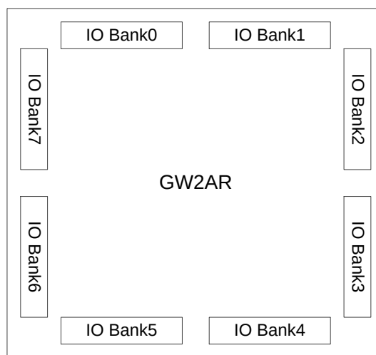
Figure 3-4 GW2ANR I/O Bank Distribution
