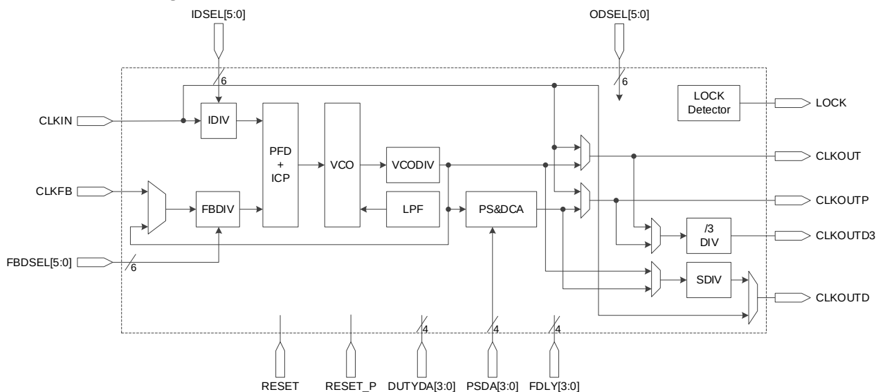
Figure 3-39 PLL Structure
