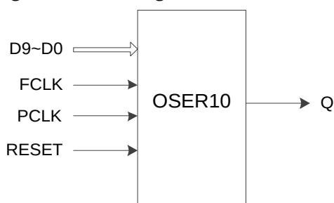
Figure 3-21 I/O Logic in OSER10 Mode
