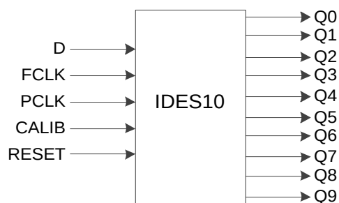
Figure 3-20 I/O Logic in IDER10 Mode
