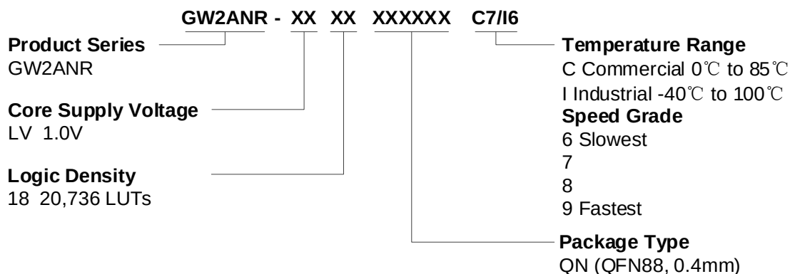
Figure 5-2 Part Naming-Production
