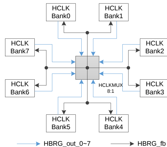
Figure 2-14 GW2A HCLK Distribution
