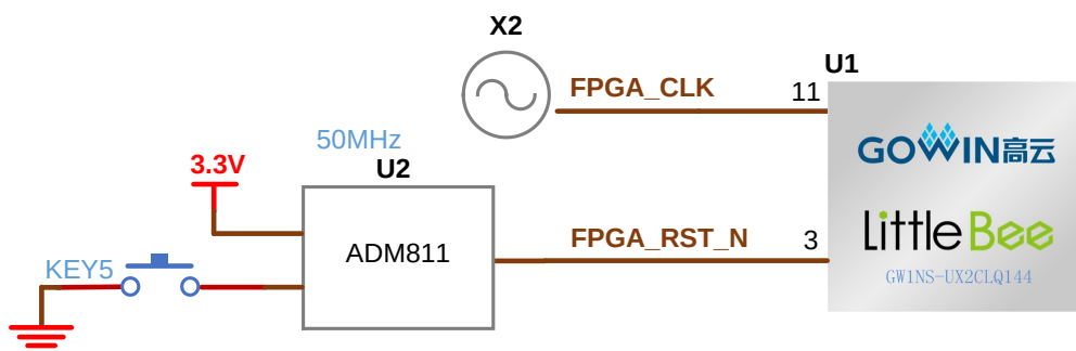
Figure 3-5 Clock, Reset
