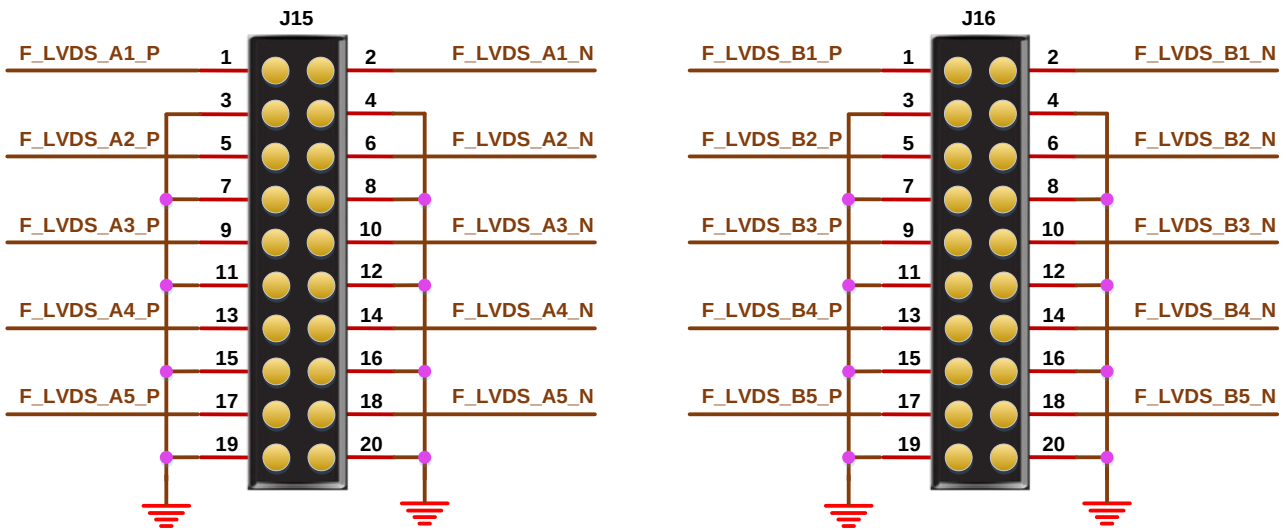
Figure 3-11 LVDS Circuit
