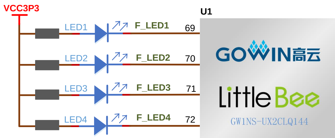
Figure 3-6 LED Circuit
