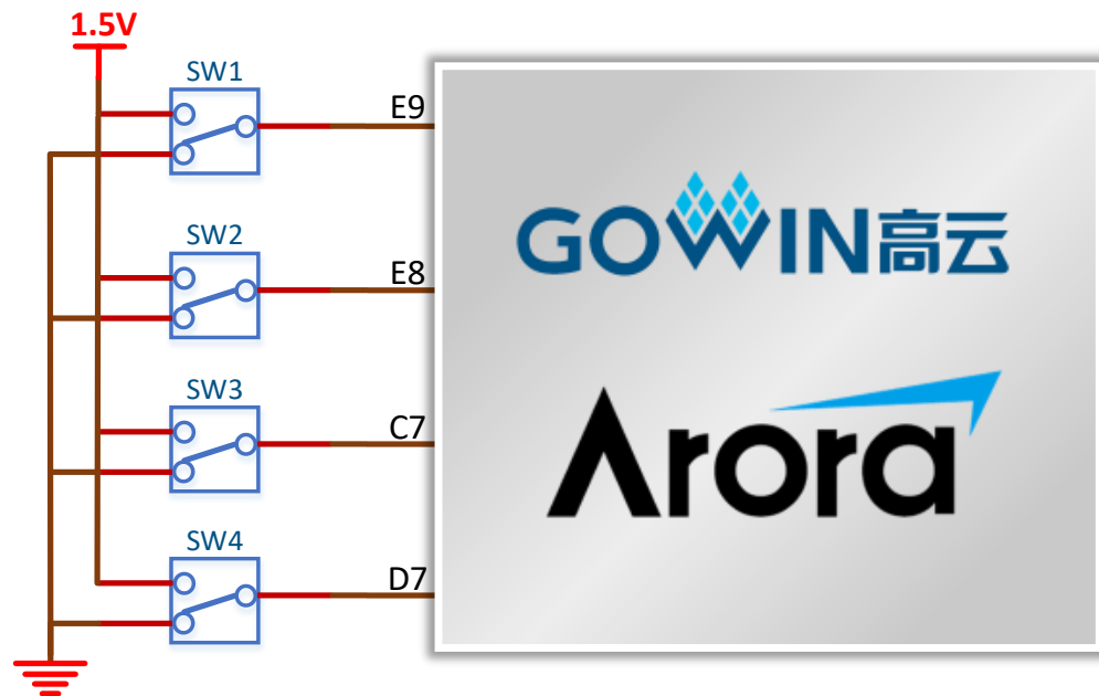
Figure 3-15 GPIO Circuit
