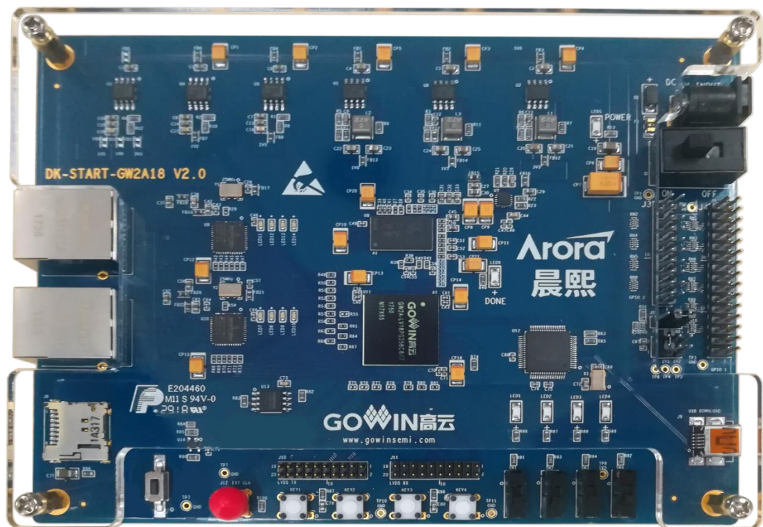
Figure 2-1 DK-START-GW2A18 V1.0
