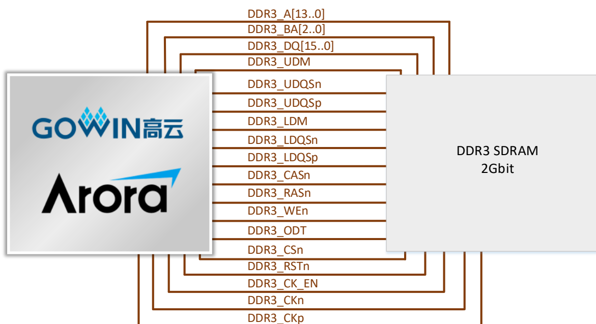
Figure 3-6 Connection Diagram of FPGA and DDR3
