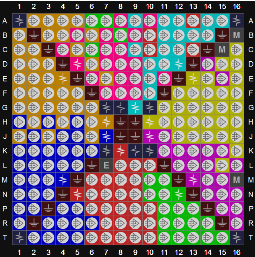
Figure 3-2 View of GW2A-18 PG256 Pins Distribution (Top View)
