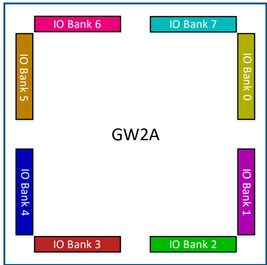
Figure 3-1 GW2A I/O Bank Distribution
