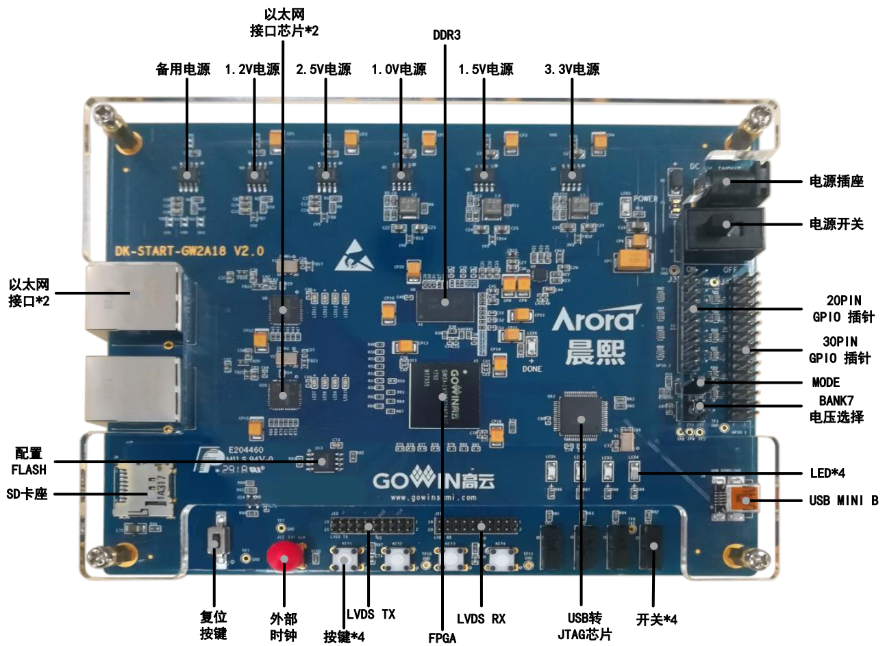
Figure 2-1 PCB Components
