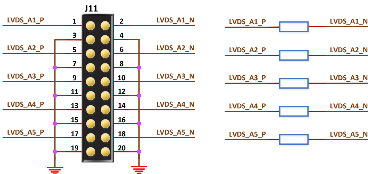
Figure 3-9 LVDS RX Interface
