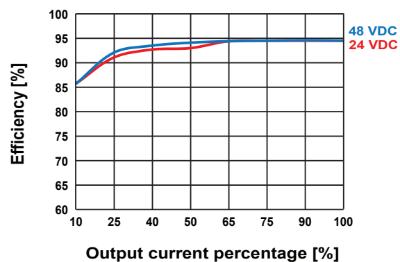
Efficiency vs. Output Load (230 VAC)
