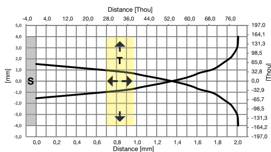
Fig. 3 Non-flush, 2mm
