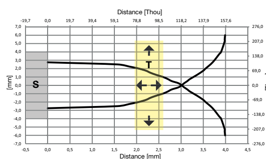
Fig. 4 Non-flush, 4mm
