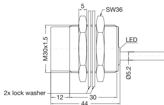
Fig. 30 Short body, non-flush version, cable
