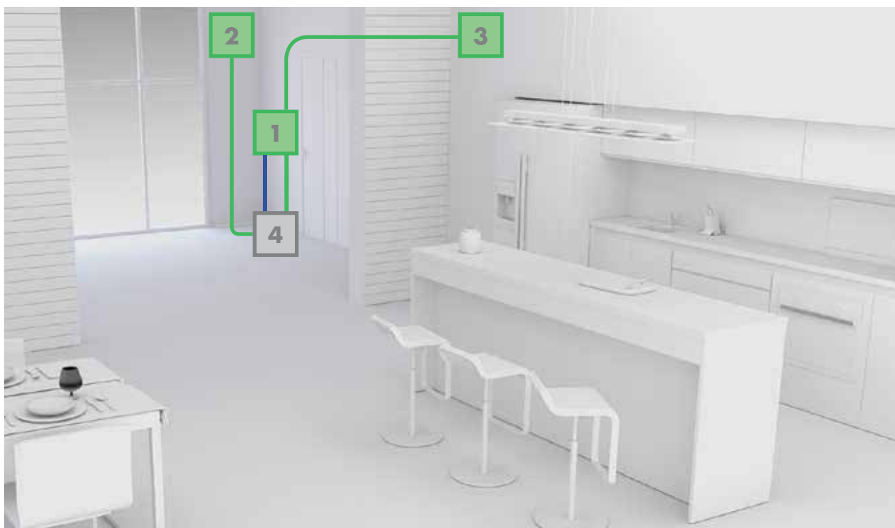
2 SHSQP360L Movement sensor with integrated luxmeter
