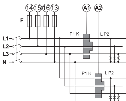
Fig. 6 Three-phase system, six single-phase circuits.
