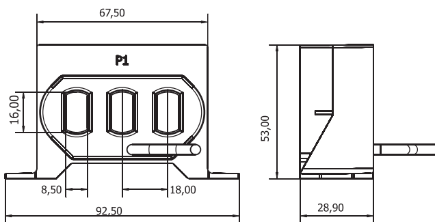
Fig. 14 TCD0W (mm)
