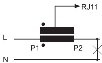
Fig. 18 Current connection
