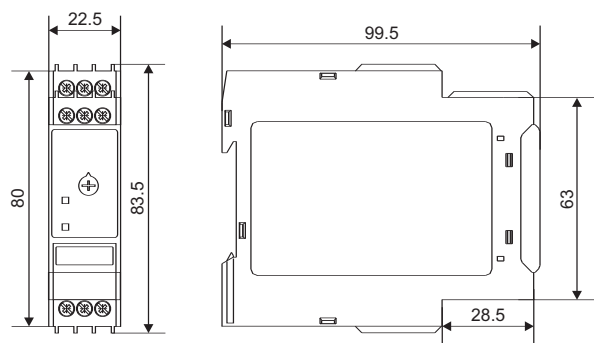
DIN-rail
