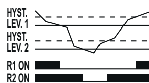
Fig. 1 Operation diagram
