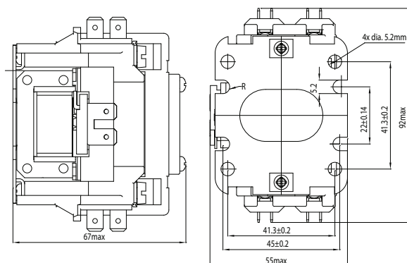
GDPx1 (1 pole+shunt)
