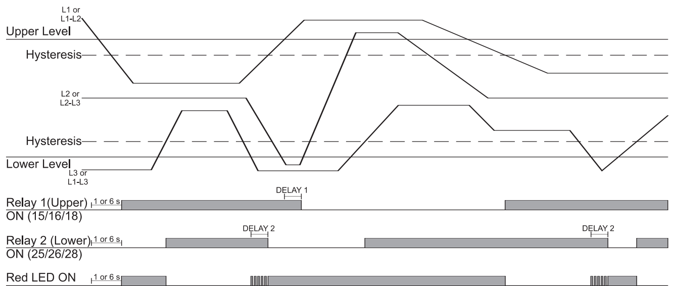
Over and undervoltage monitoring (2 x SPDT relays)
