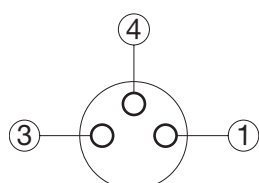
Fig. 7 3-wire
