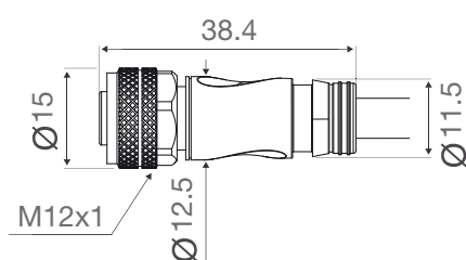
Fig. 5 Straight
