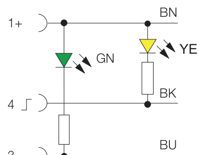
Fig. 13 3-wire, NPN
