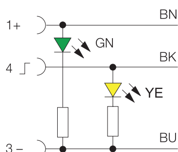
Fig. 12 3-wire, PNP
