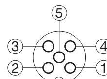
Fig. 11 5-wire
