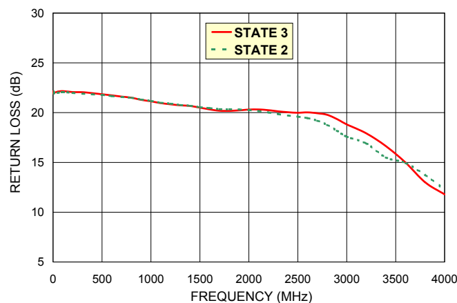
RF COM RETURN LOSS Vs. FREQUENCY @ +25°C
