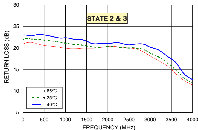
RF COM RETURN LOSS Vs. FREQUENCY
