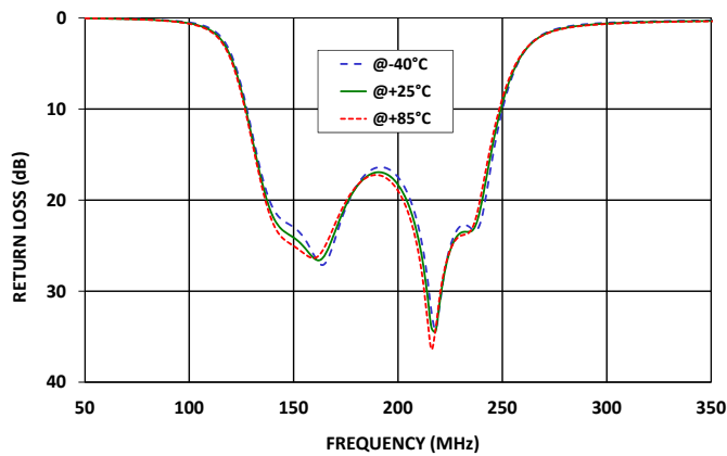
ZX75BP-188-S+ RETURN LOSS
