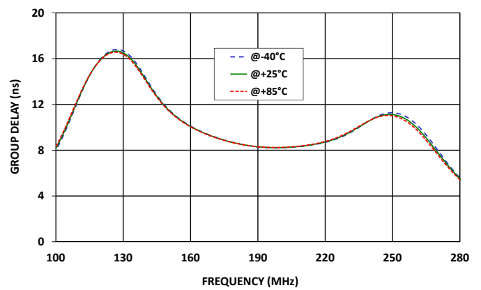
ZX75BP-188-S+ GROUP DELAY
