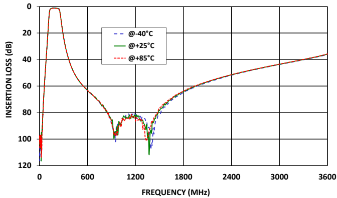
ZX75BP-188-S+ INSERTION LOSS
