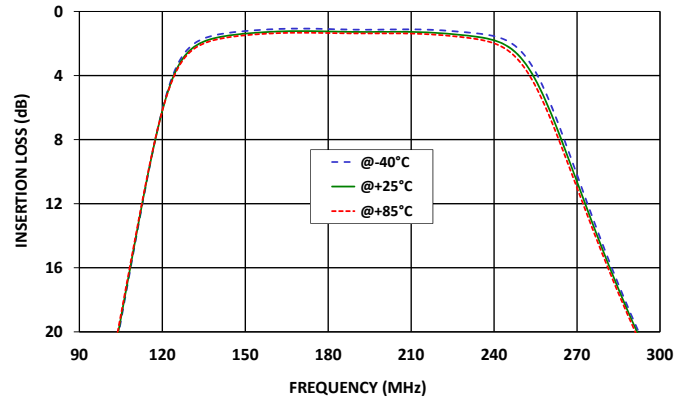
ZX75BP-188-S+ INSERTION LOSS (Zoomed)
