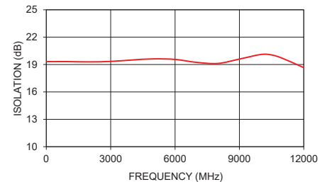
ZFRSC-123-S+ ISOLATION
