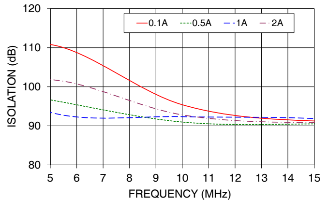
Z4BT-2R15G+ REF to RF port ISOLATION WITH CURRENT ( P_{in} = 0\text{dBm} )
