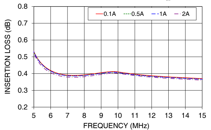
Z4BT-2R15G+ REF to Common port INSERTION LOSS WITH CURRENT ( P_{in} = 0\text{dBm} )
