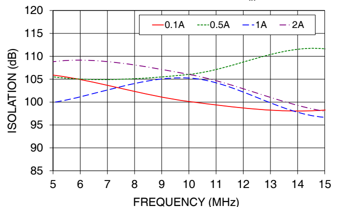
Z4BT-2R15G+ RF to DC port ISOLATION WITH CURRENT ( P_{in} = 0\text{dBm} )
