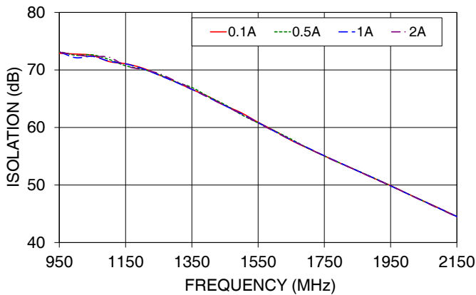
Z4BT-2R15G+ RF to REF port ISOLATION WITH CURRENT ( P_{in} = 0\text{dBm} )
