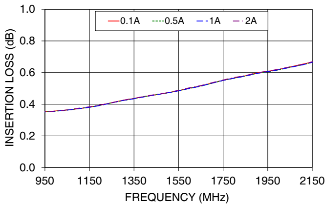
Z4BT-2R15G+ RF to Common port INSERTION LOSS WITH CURRENT ( P_{in} = 0\text{dBm} )
