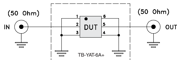
Fig 1. Block diagram of Test Circuit used for characterization, Test board TB-YAT-6A+ Conditions: Attenuation, VSWR: Pin=-10 dBm
