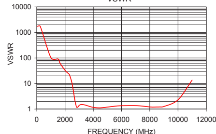
VHF-2700A+ VSWR
