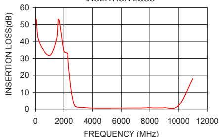
VHF-2700A+ INSERTION LOSS
