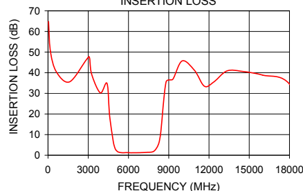
VBFZ-6260+ INSERTION LOSS
