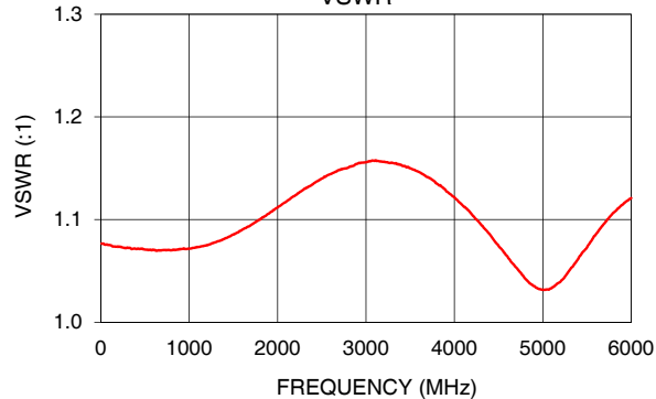
UNAT-1A+ VSWR
