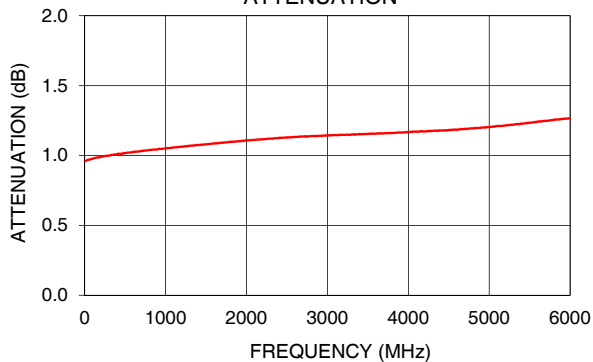
UNAT-1A+ ATTENUATION
