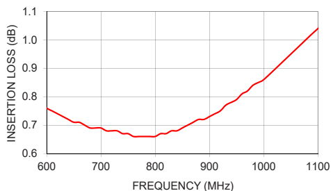
TCN3-11+ INSERTION LOSS
