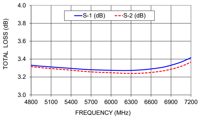
SCW-2-722+ TOTAL LOSS
