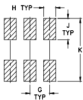
Suggested Layout, Tolerance to be within ±.002
