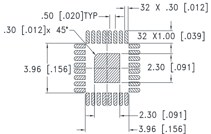
PCB Land Pattern
