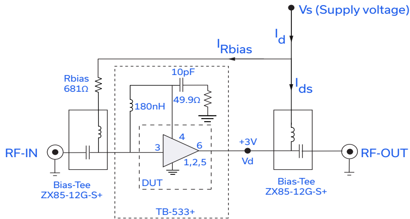
Fig 1. Block Diagram of Test Circuit used for characterization. (DUT soldered on Mini-Circuits Characterization Test Board TB-533+) Gain, Output power at 1dB compression (P1 dB), output IP3 (OIP3) and Noise Figure measured using Agilent's N5242A PNA-X microwave network analyzer.
