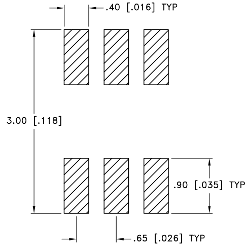
Suggested Layout Tolerance to be within \pm .002
