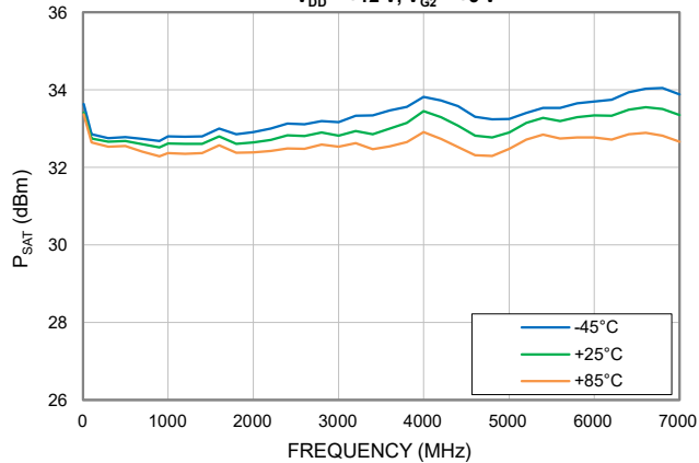
P_{SAT} vs. TEMPERATURE, V_{DD} = +12 V, V_{G2} = +5 V
