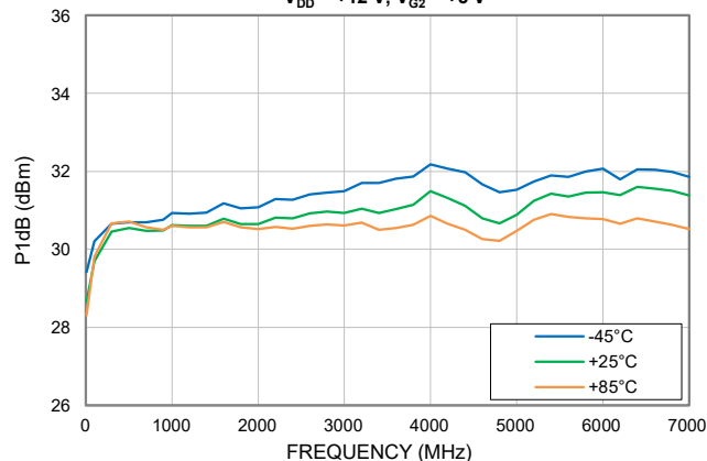
P1dB vs. TEMPERATURE, V_{DD} = +12 V, V_{G2} = +5 V
