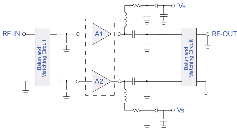
Fig 2. Recommended Application Circuit. Refer to following Mini-Circuits Evaluation Boards for parts list. 50Ω: TB-566-50H+ 75Ω: TB-566-75H+ TB-666-50H+
