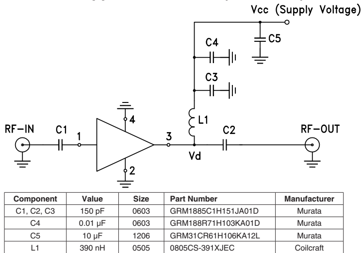
Fig 2. Test board (TB-869A+) includes case, connectors, and components soldered to PCB
