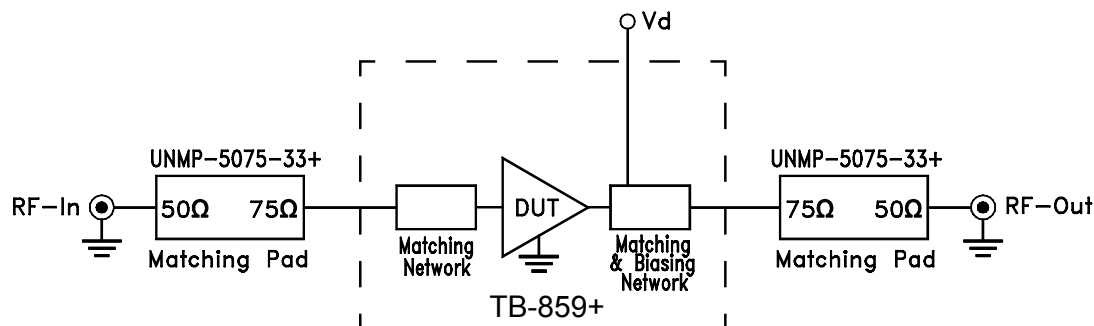
Fig 1. Block Diagram of Test Circuit used for characterization. (DUT tested on Mini-Circuits Characterization Eval board TB-859+) Gain, Return loss, Output power at 1dB compression (P1 dB), output IP3 (OIP3), output IP2 (OIP2) and noise figure measured using Agilent's N5242A PNA-X microwave network analyzer.
