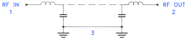
Figure 1. LFCV-1752+ Functional Diagram
