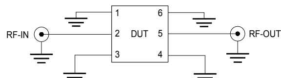
Fig 1. Block diagram of Test Circuit used for characterization, Test board TB-934-4C+ Conditions: Attenuation, VSWR: Pin=0 dBm
