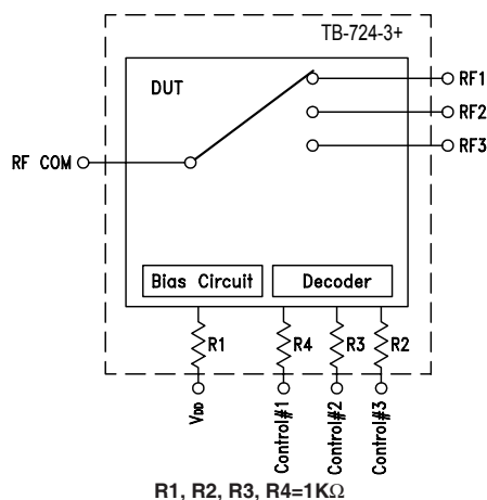
Figure 1: Block Diagram Of Test Circuit Used For Characterization. (DUT soldered on Mini-Circuits' TB-724-3+)
