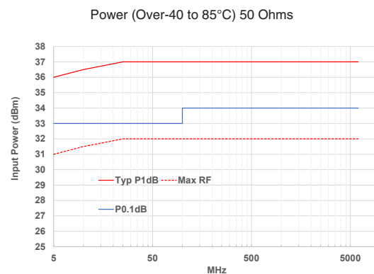
Figure 2. Max RF( operating), P_{0.1\text{dB}} (Typ) and P_{1\text{dB}} (Typ) vs frequency.
