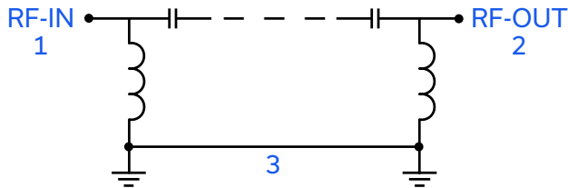
Figure 1. HFCU-1682+ Functional Diagram
