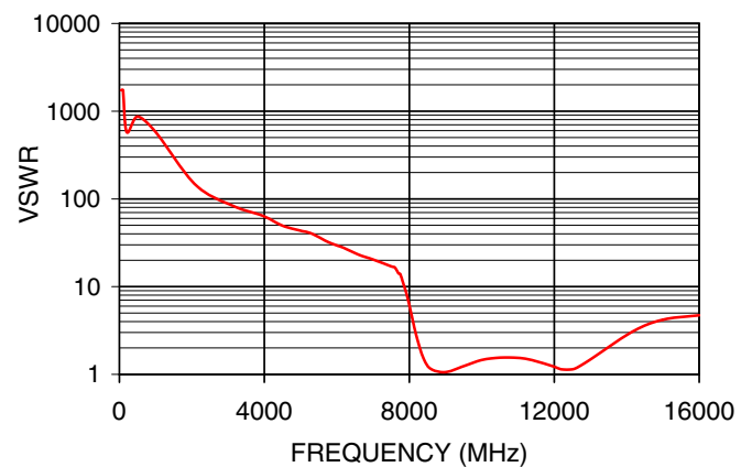
HFCN-8400D+ VSWR
