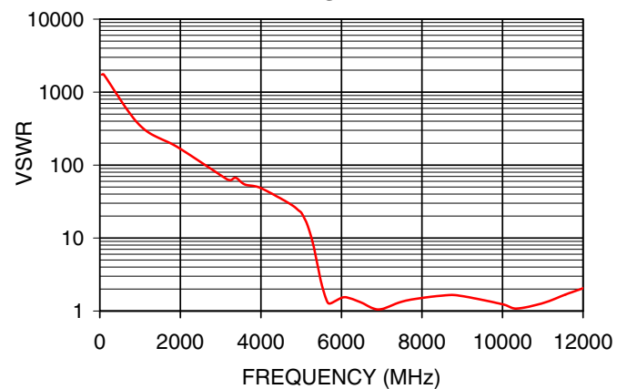
HFCN-5500D+ VSWR
