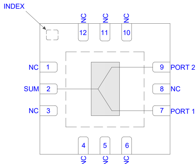
Figure 1. GP2X1A+ Functional Diagram
