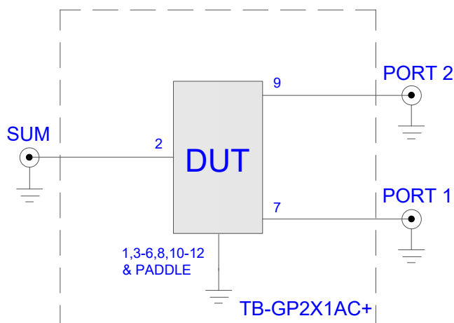
Figure 2. GP2X1A+ Characterization and Application Circuit.
