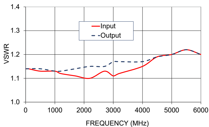
EQY-8-63+ VSWR
