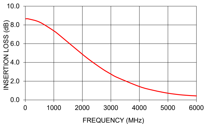
EQY-8-63+ INSERTION LOSS
