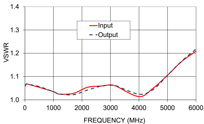
EQY-10-63+ VSWR
