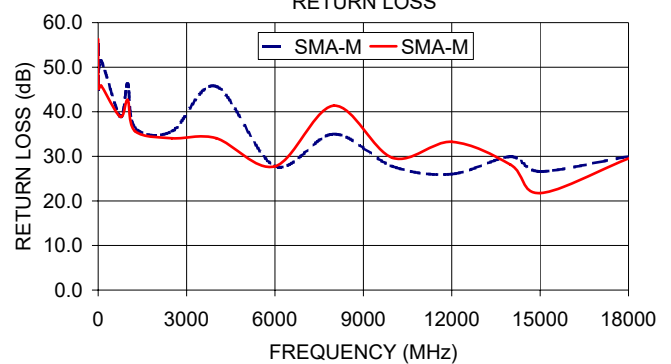
CBL-4FT-SMSM+ RETURN LOSS
