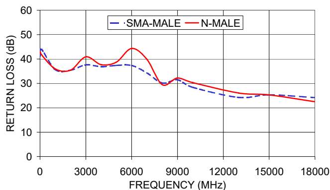
CBL-2FT-SMNM+ RETURN LOSS
