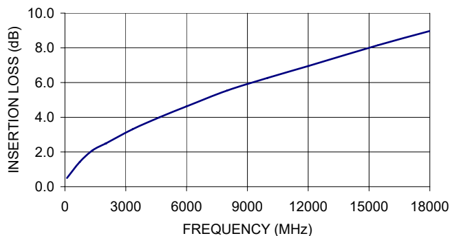
CBL-15FT-SMSM+ INSERTION LOSS
