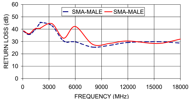
CBL-15FT-SMSM+ RETURN LOSS
