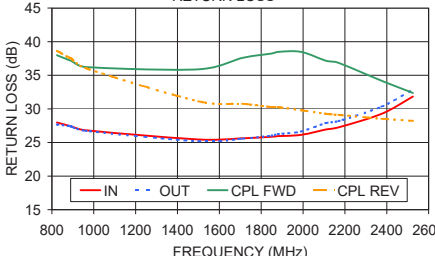
BDCN-7-25+ RETURN LOSS
